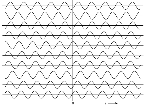
(b) Uniform phase
